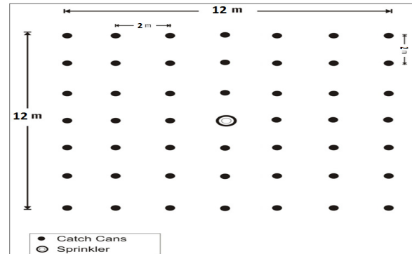
Fig. 1: Layout of Catch-Cans around a Sprinkler Head
