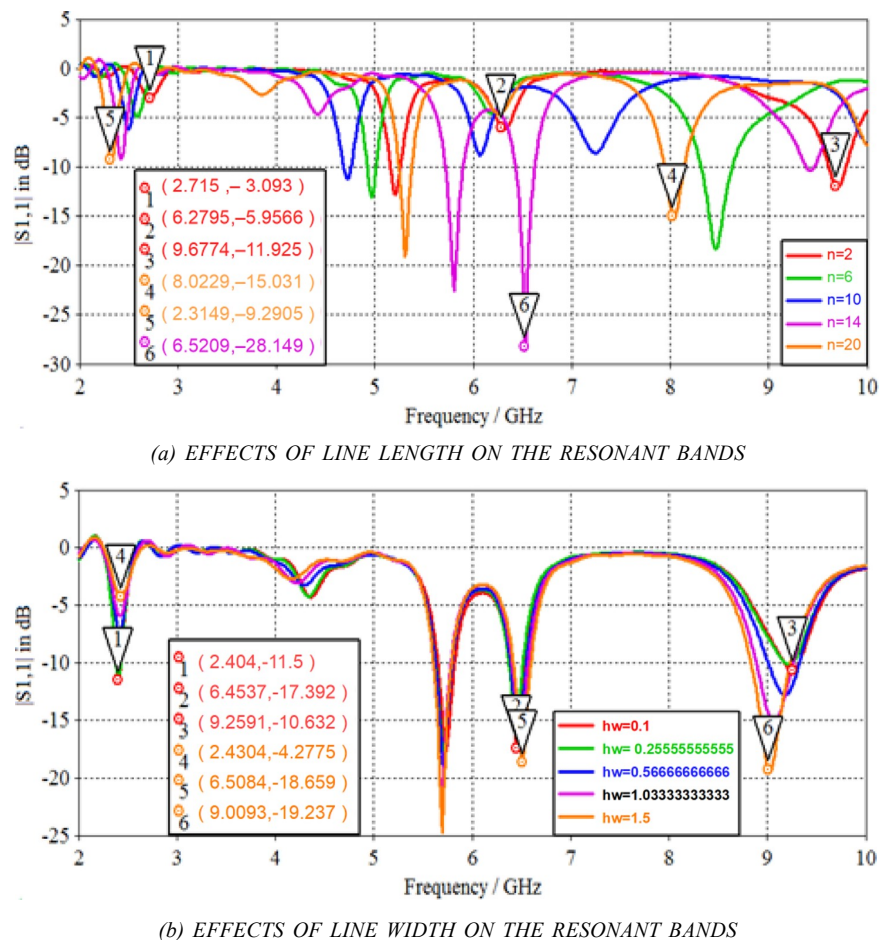
FIG. 7. VARIATIONS OF RESONANT FREQUENCY BANDS WITH RESPECT TO DIFFERENT DIMENSIONS OF MICROSTRIP FEED LINE OF PROPOSED FRACTAL PATCH ANTENNA
