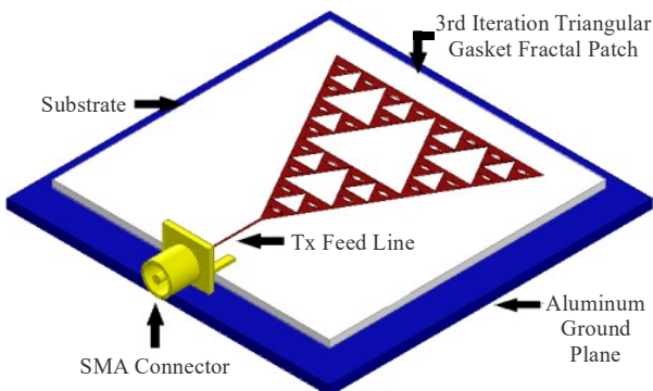
FIG. 1. PROPOSED 3D ARCHITECTURE OF THIRD ORDER DIAGONAL SLOT EMBEDDED TRIANGULAR GASKET FRACAL PATCH ANTENNA LABELED PERSPECTIVE VIEW
