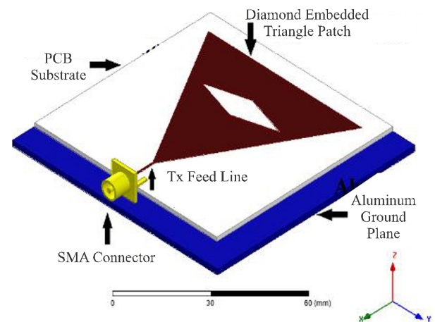
(a) LABELED PERSPECTIVE VIEW
