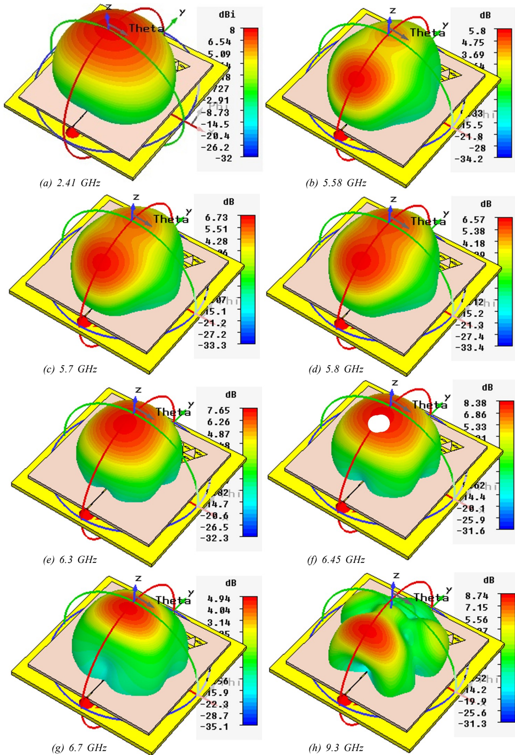
FIG. 11. CST GAIN PLOTS OF PROPOSED THIRD ORDER SLOT EMBEDDED TRIANGULAR GASKET FRAGMENTAL PATCH ANTENNA AT FREQUENCIES
