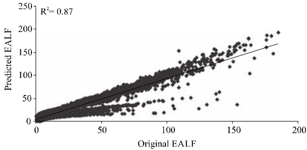
FIG 8(b). ILLUSTRATION OF ACTUAL VERSUS PREDICTED, VALIDATION DATA OF AXLE TRUCK TYPE-3
