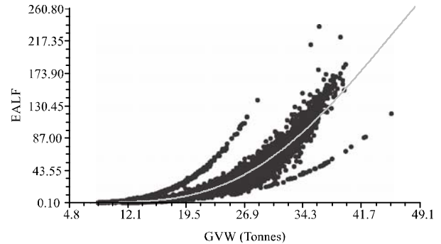
FIG. 7(a). REGRESSION PLOT OF AXLE TRUCK TYPE-2
