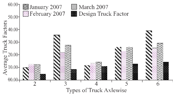
FIG. 6(B). COMPARISON OF AVERAGE TRUCK FACTOR AND DESIGN TRUCK FACTOR MULLAH MANSOOR WEIGHING STATION, JANUARY TO MARCH 2007
