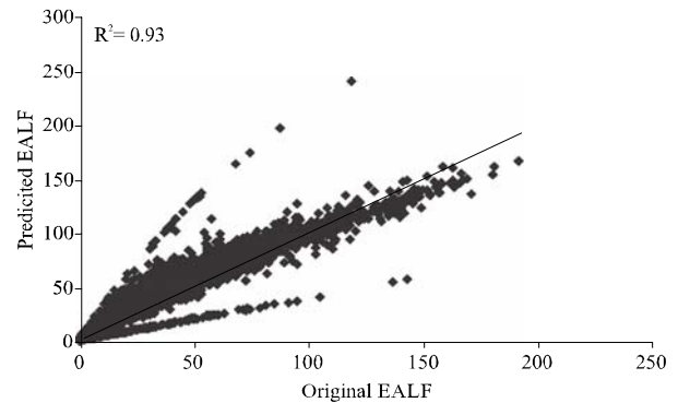
FIG.7(b). ILLUSTRATION OF ACTUAL VERSUS PREDICTED, VALIDATION DATA OF AXLE TRUCK TYPE-2
