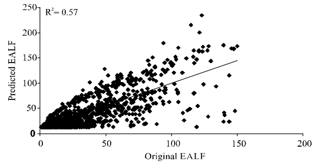
FIG 10(b). ILLUSTRATION OF ACTUAL VERSUS PREDICTED, VALIDATION DATA OF AXLE TRUCK TYPE-5
