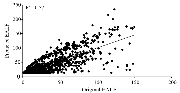
FIG 11(a). REGRESSION PLOT OF AXLE TRUCK TYPE-6
