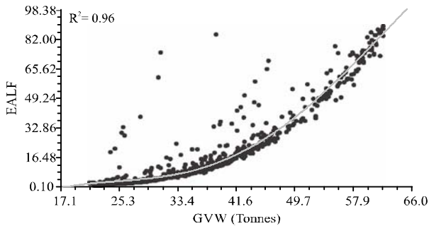
FIG 9(a). REGRESSION PLOT OF AXLE TRUCK TYPE-4
