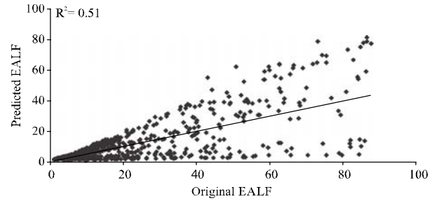
FIG.10(a). REGRESSION PLOT OF AXLE TRUCK TYPE-5
