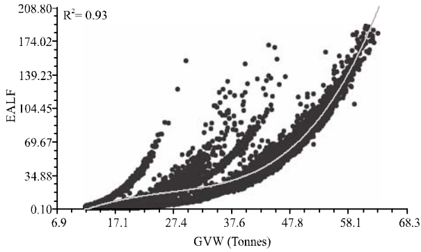
FIG 8(a). REGRESSION PLOT OF AXLE TRUCK TYPE-3
