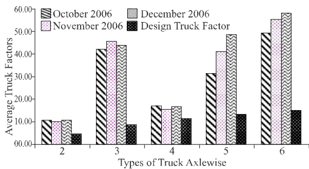
FIG. 6(a). COMPARISON OF AVERAGE TRUCK FACTOR AND DESIGN TRUCK FACTOR MULLAH MANSOOR WEIGHING STATION, OCTOTOBER TO DECEMBER 2006
