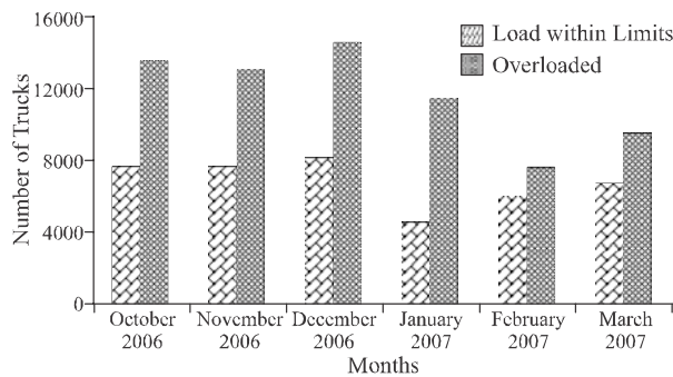
FIG. 5. LOADED VERSUS OVERLOADED (MULLAH MANSOOR WEIGHING STATION)
