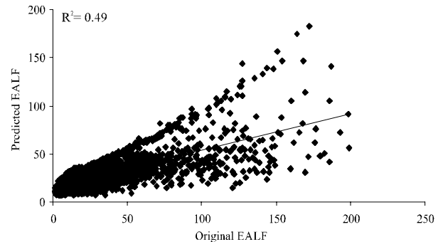
FIG 11(b). ILLUSTRATION OF ACTUAL VERSUS PREDICTED, VALIDATION DATA OF AXLE TRUCK TYPE-6
