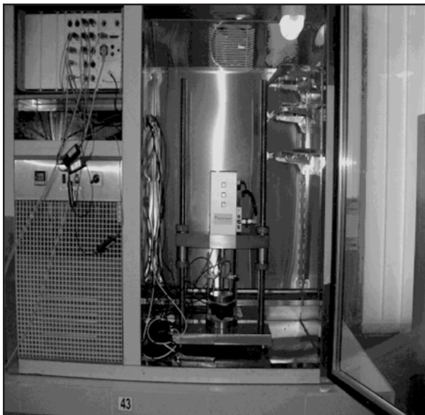
FIG. 2. UNIVERSAL TESTING MACHINE (UTM-5P)
