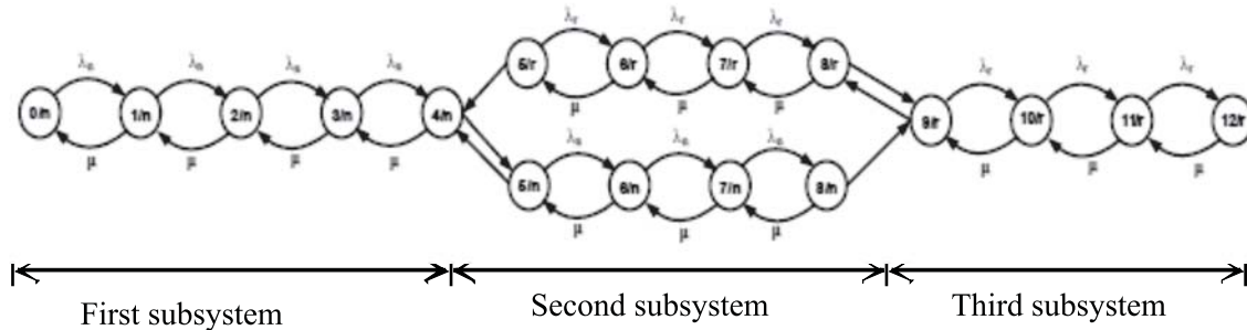
FIG. 3. SIMPLIFIED STRUCTURED MARKOV CHAIN
