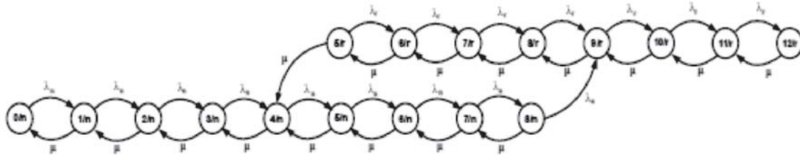
FIG. 2. STRUCTURED MARKOV CHAIN: S_{go} = 4, S_{stop} = 9 AND S = 12
