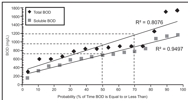
FIG. 1. STATISTICAL DISTRIBUTION OF TOTAL AND SOLUBLE BOD FOR RAW NISHAT WASTEWATER
