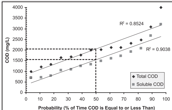
FIG. 2. STATISTICAL DISTRIBUTION OF TOTAL AND SOLUBLE COD FOR RAW UNSETTLED NISHAT WASTEWATER
