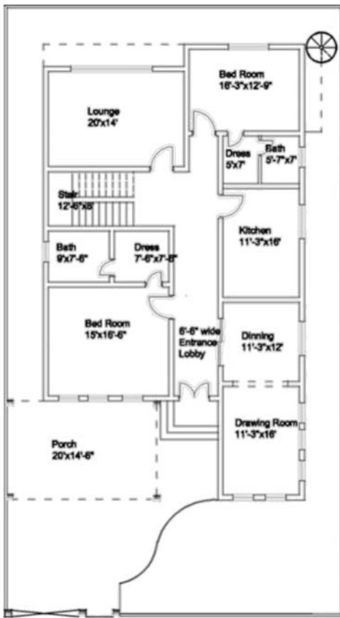
FIG. 2(a). ARCHITECTURAL PLAN (GROUND FLOOR)
