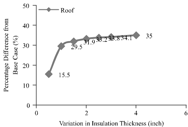
FIG. 4. PERCENTAGE DIFFERENCE OF ROOF INSULATION VARIATIONS FROM BASE CASE
