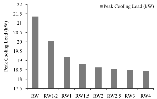
FIG. 5. COMPARISON OF PEAK COOLING LOADS BY MODIFICATIONS IN WALL
