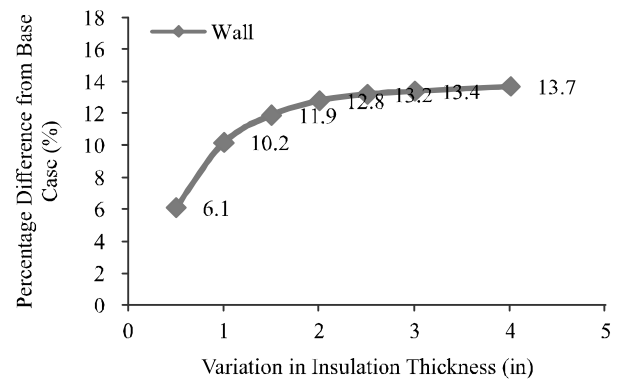
FIG. 6. PERCENTAGE DIFFERENCE OF WALL INSULATION VARIATIONS FROM BASE CASE
