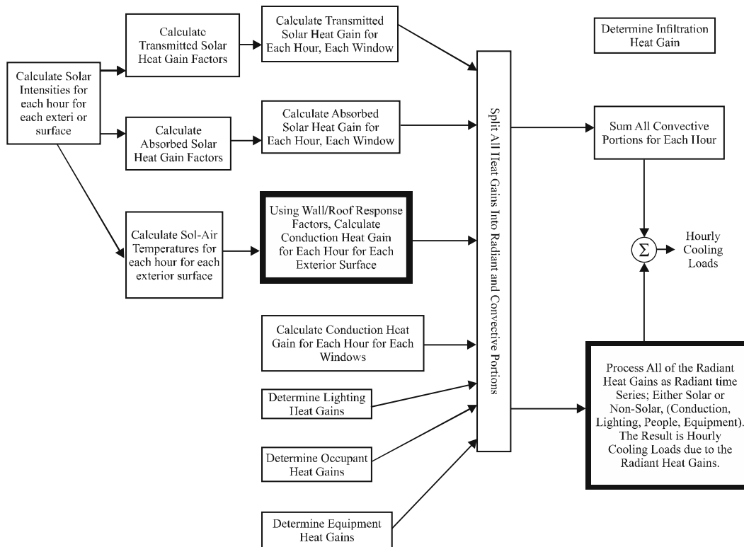
FIG. 1. OVERVIEW OF RADIANT TIME SERIES METHOD [13]
