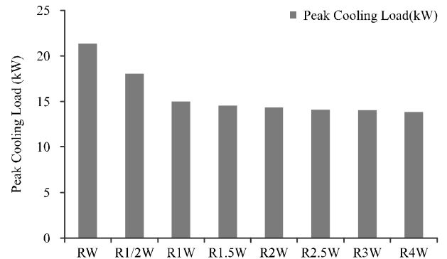
FIG. 3. COMPARISON OF PEAK COOLING LOADS BY MODIFICATIONS IN ROOF
