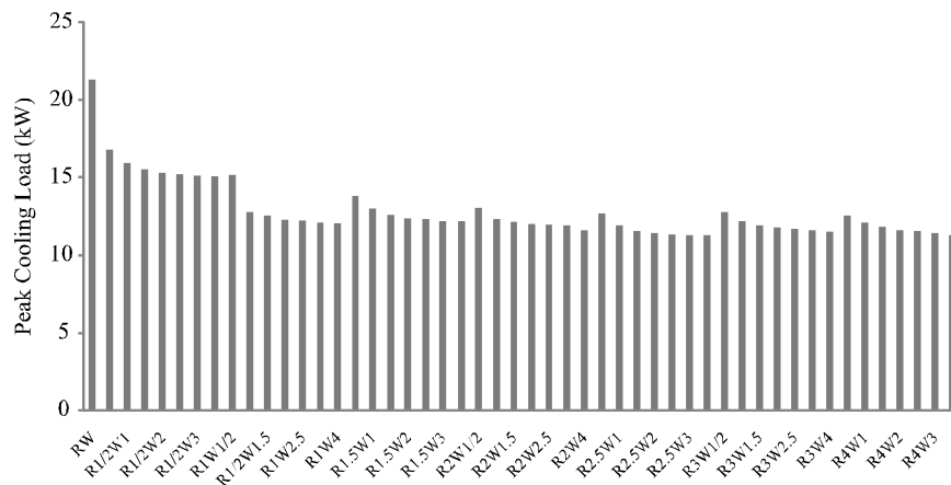
FIG. 7. COMPARISON OF PEAK COOLING LOADS BY MODIFICATIONS IN BOTH WALL AND ROOF
